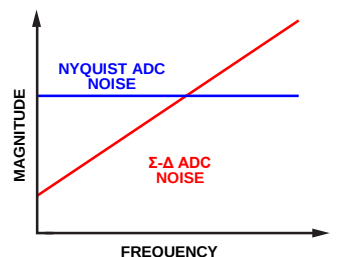
Figure 17. Noise Performance for Nyquist Rate and \Sigma\text{-}\Delta ADCs
