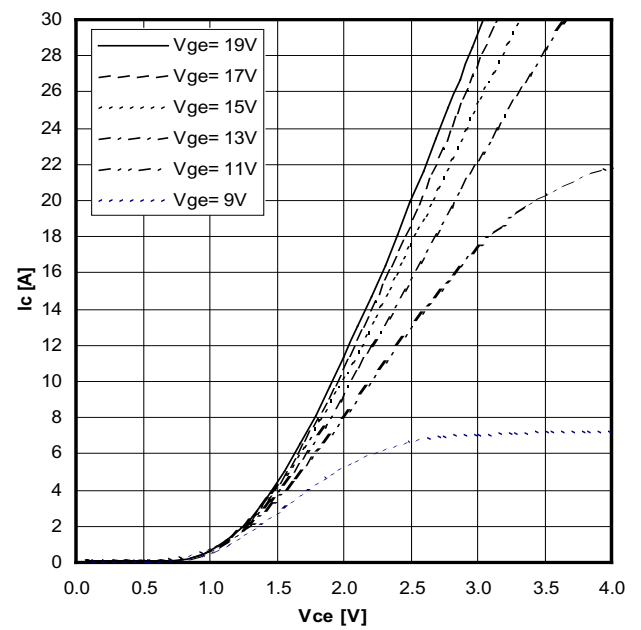
Typical output characteristics ( 125\text{ °C} )
