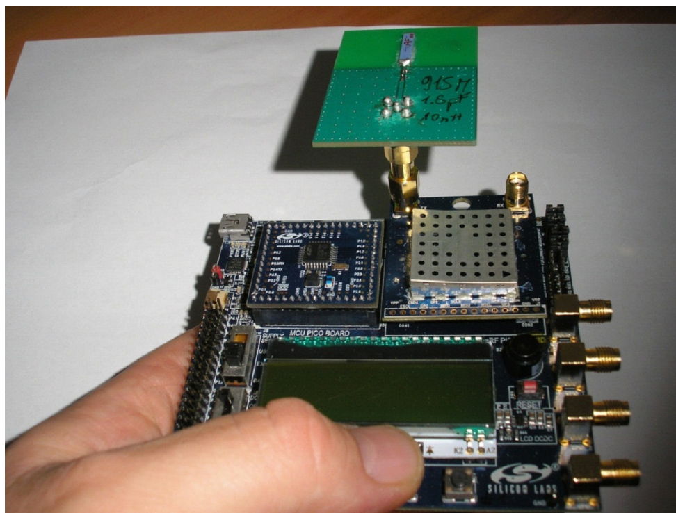
Figure 83. Figure 6.4. Typical hand effect on the main board during impedance and range measurement
