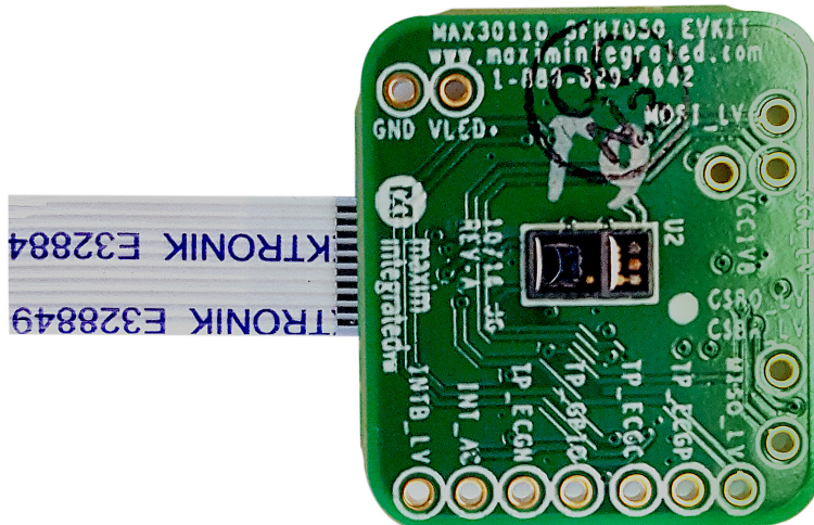
Figure 9. MAX30110 EV Kit—Hardware Setup (Sensor PCB 2 – Top View)
