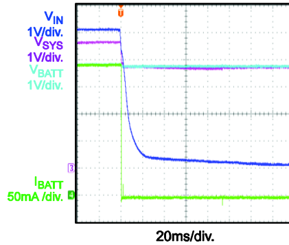
EN On @ Input Current Limit Based PPM
