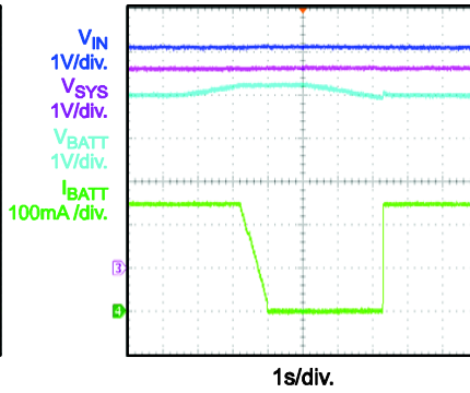
Supplement Mode Steady State V_{BATT}=3.7V, I_{SYS}=600mA
