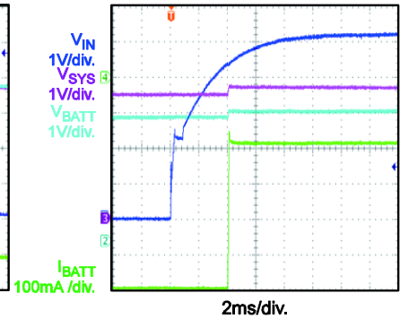
EN Off @ Input Current Limit Based PPM
