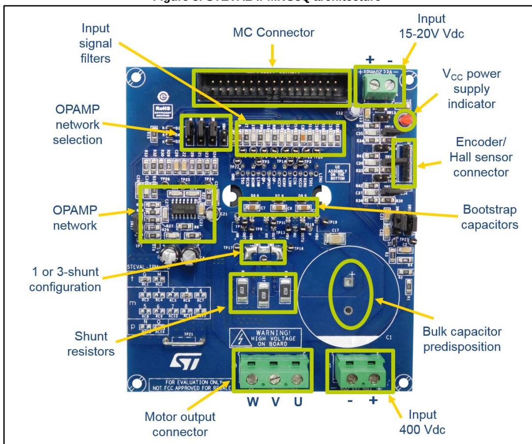
Figure 8: STEVAL-IPMNG3Q architecture
