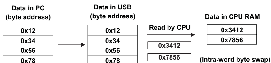
Figure 4. CPU Read From USB
