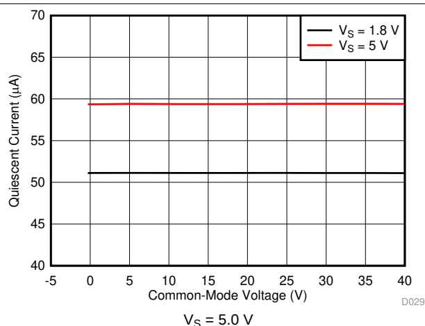
Figure 10. Quiescent Current vs Common Mode Voltage
