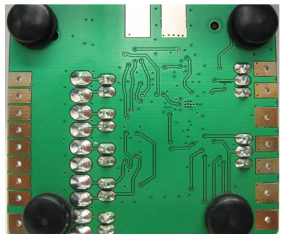
Figure 2. SSM2304 Evaluation Board Typical Setup
