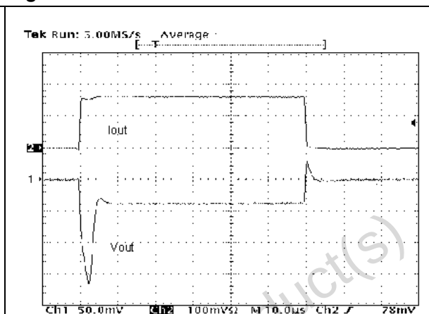
Figure 16. Load transient
