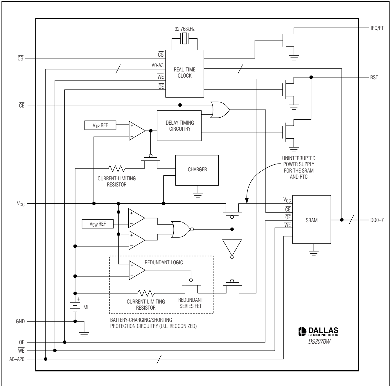
Functional Diagram
