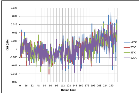
FIGURE 40-61: Typical DAC DNL Error, VDD = 3.0V, VREF = External 3.0V.
