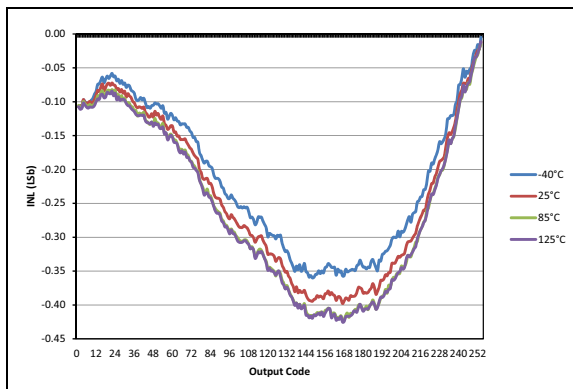
FIGURE 40-62: Typical DAC INL Error, VDD = 3.0V, VREF = External 3.0V.
