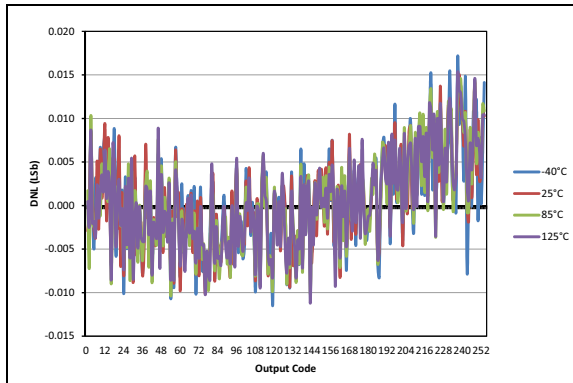
FIGURE 40-63: Typical DAC DNL Error, VDD = 5.0V, VREF = External 5.0V PIC16F19195/6/7 Only.
