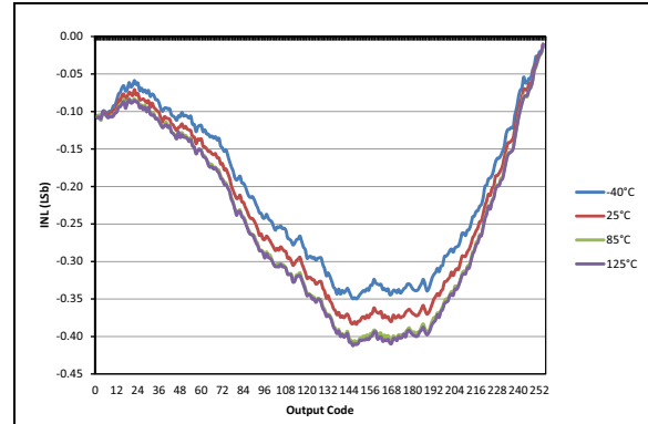
FIGURE 40-64: Typical DAC INL Error, VDD = 5.0V, VREF = External 5.0V PIC16F19195/6/7 Only
