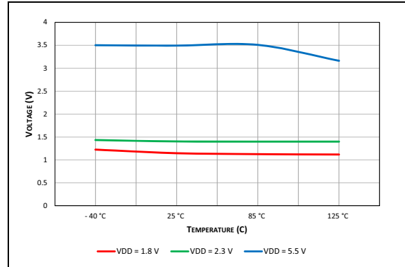
FIGURE 40-94: Typical Input High Voltage with I^2C Level.
