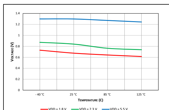
FIGURE 40-95: Typical Input Low Voltage with SMBus Level.
