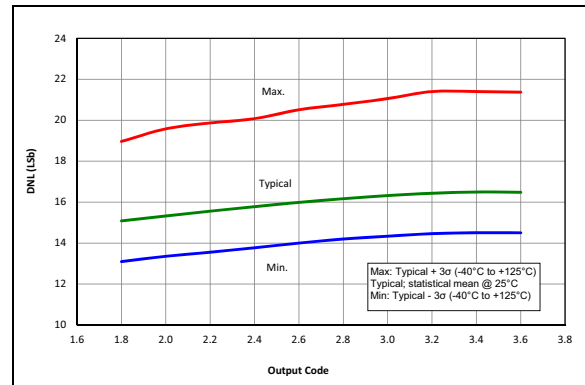
FIGURE 40-65: DAC DNL Error, VDD = 3.0V, PIC16LF19195/6/7 Only.
