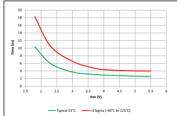
FIGURE 40-100: Fall Time, Slew Rate Control Disabled.
