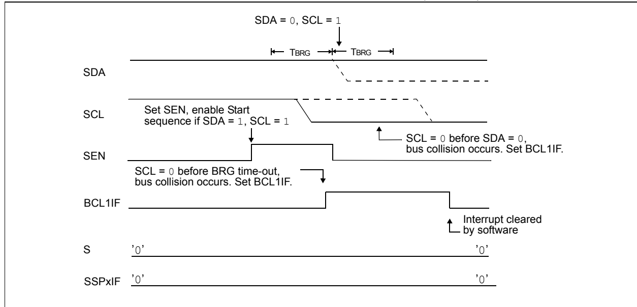
FIGURE 33-35: BRG RESET DUE TO SDA ARBITRATION DURING START CONDITION
