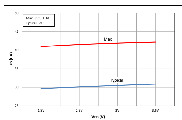
FIGURE 40-18: IPD, Comparator C1, PIC16LF19195/6/7 Only.
