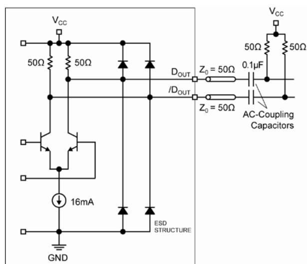
Figure 3. Output Structure
