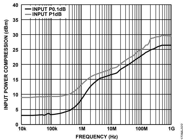
Figure 22. Input P0.1dB and Input P1dB vs. Frequency over Temperature, V_{DD} = 3\text{ V} , Low Frequency Detail
