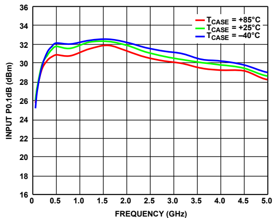
Figure 14. Input 0.1 dB Power Compression (P0.1dB) vs. Frequency over Temperature, V_{DD} = 5\text{ V}
