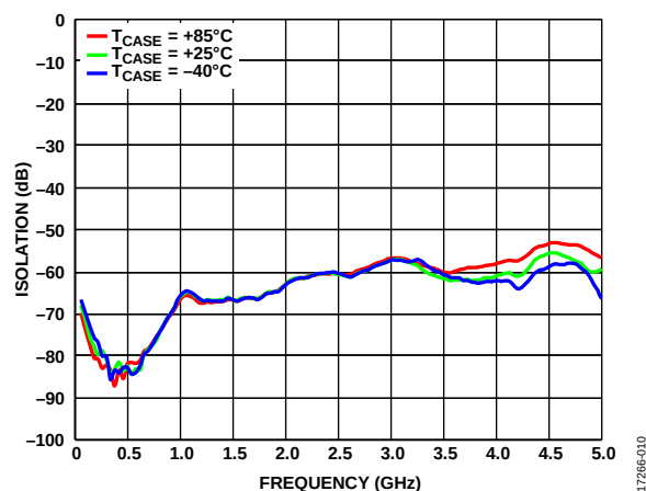
Figure 10. Isolation Between RFC and RF2 vs. Frequency over Temperature
