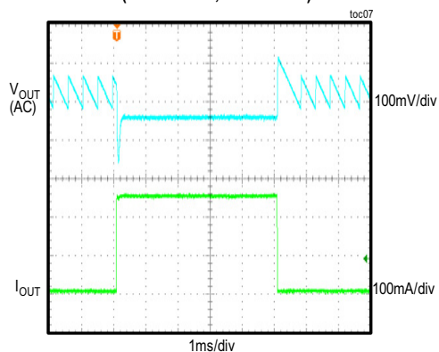
MAX17761, LOAD CURRENT STEPPED FROM 0A TO 0.25A (5V OUTPUT, PFM MODE)
