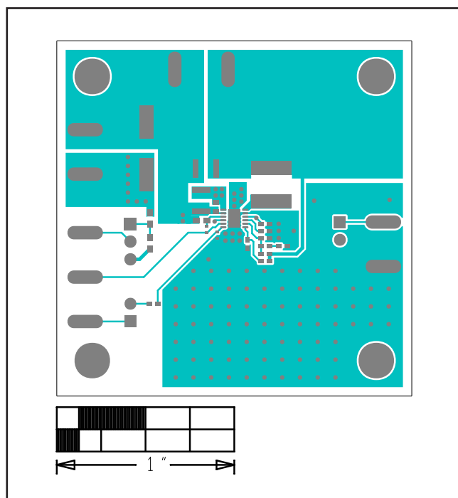
MAX17761 EV Kit PCB 5V Output Top Layer
