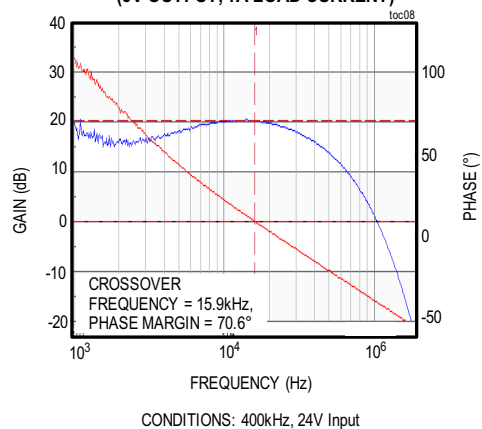
MAX17761, BODE PLOT (5V OUTPUT, 1A LOAD CURRENT)
