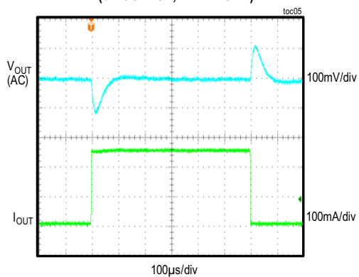
MAX17761, LOAD CURRENT STEPPED FROM 0A TO 0.25A (5V OUTPUT, PWM MODE)
