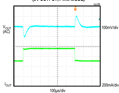
MAX17761, LOAD CURRENT STEPPED FROM 0.5A TO 0.75A (5V OUTPUT, PWM MODE)
