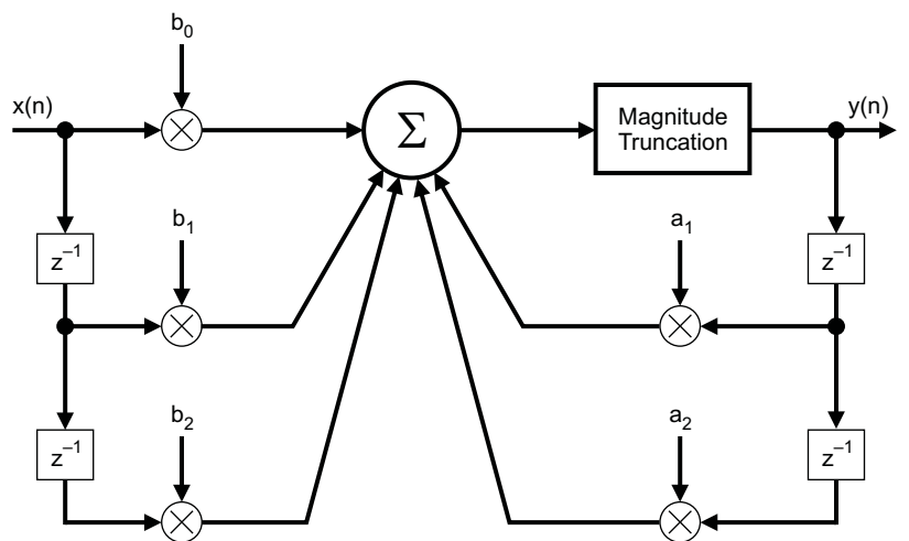
Figure 34. BiQuad Filter
