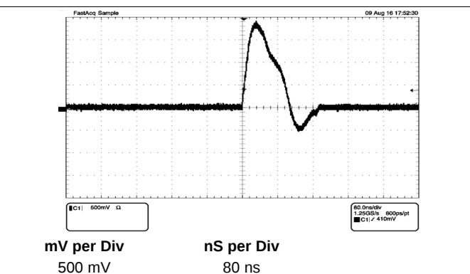
Figure 18. 10BASE-Tc Link Pulse Waveform
