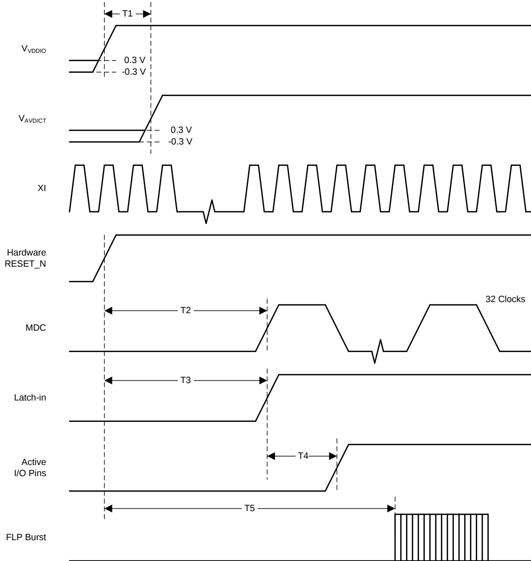
Figure 1. Power-Up Timing
