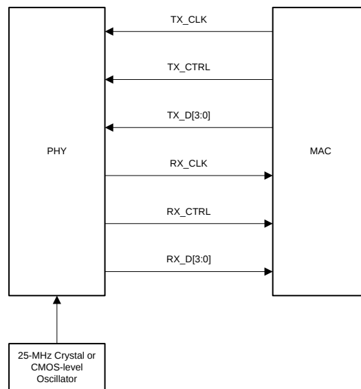
Figure 27. RGMII Signaling
