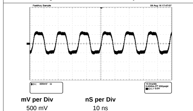
Figure 19. 100BASE-FX Waveform
