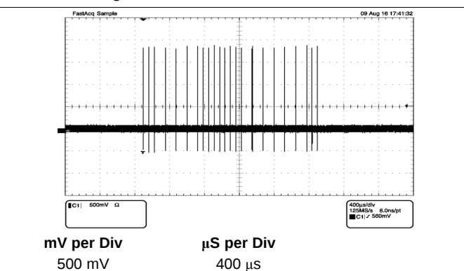
Figure 20. Auto-Negotiation Fast Link Pulses Waveform
