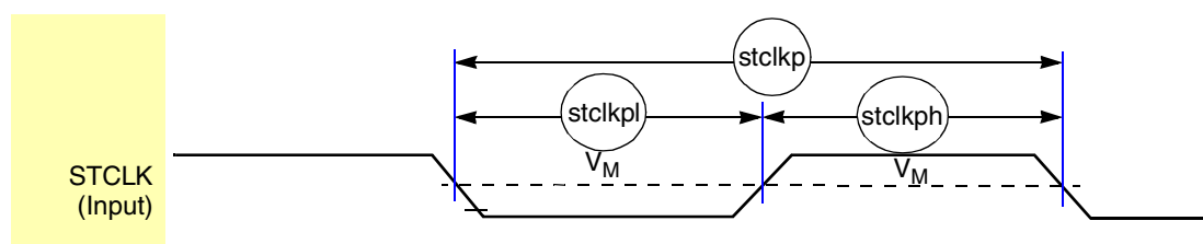
Figure 92. STCLK Timing
