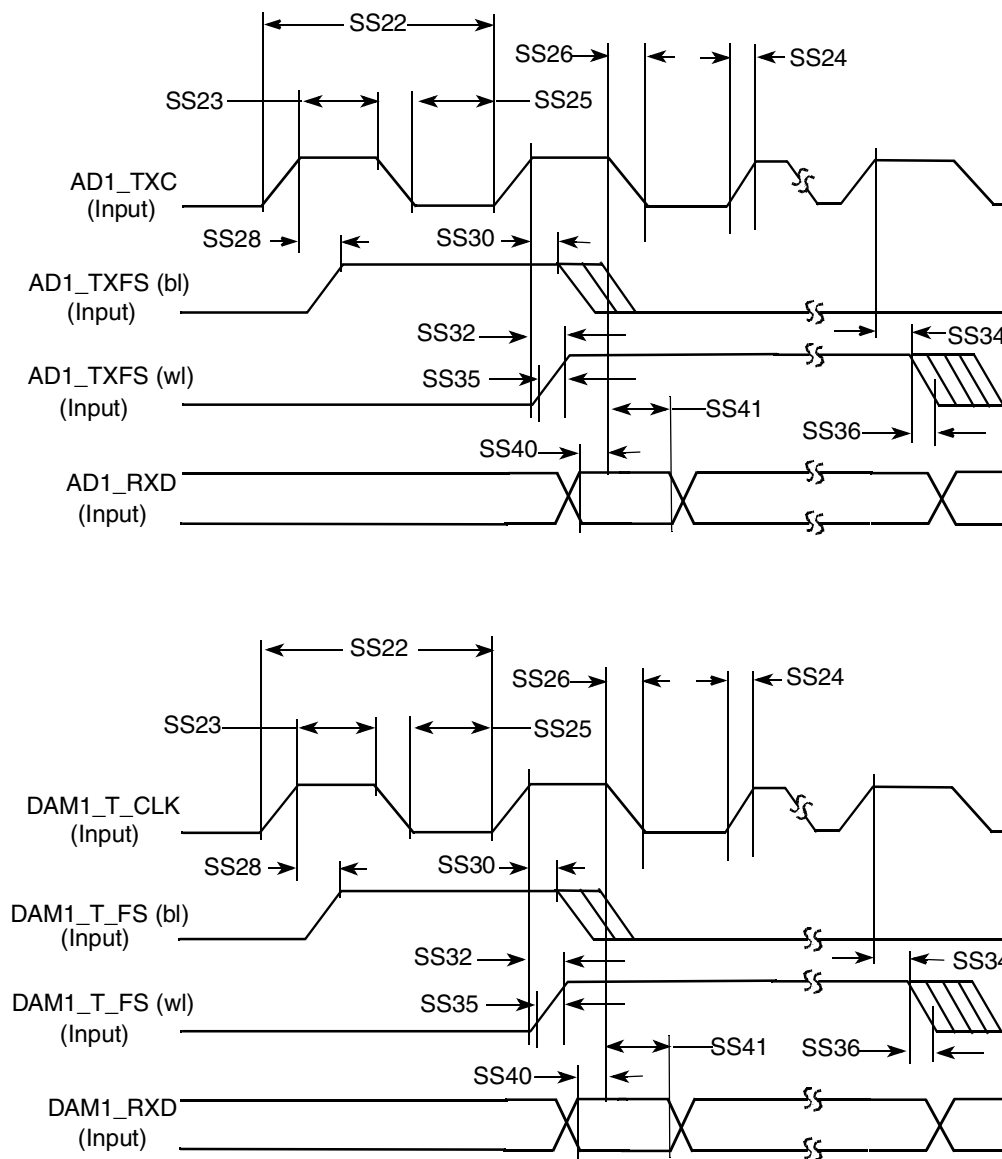
Figure 96. SSI Receiver with External Clock Timing Diagram
