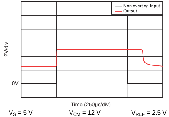
图 20. Noninverting Differential Input Overload
