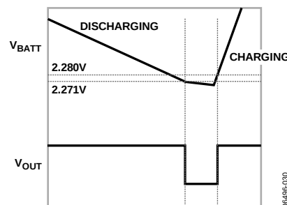
Figure 3. Li-Ion Monitoring Waveforms
