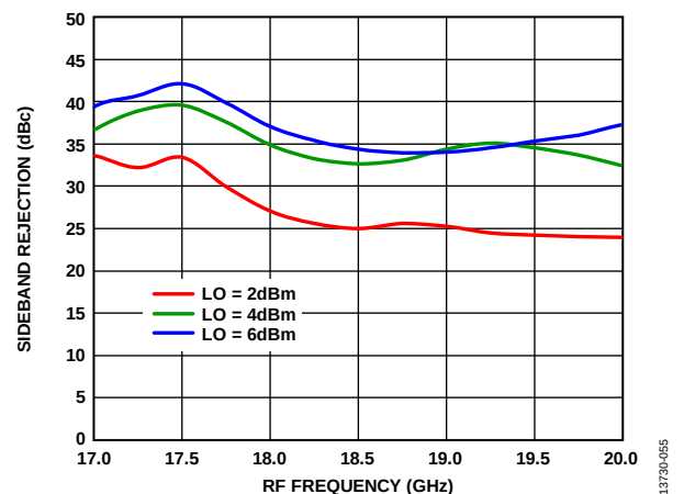
Figure 55. Sideband Rejection vs. RF Frequency at Various LO Powers
