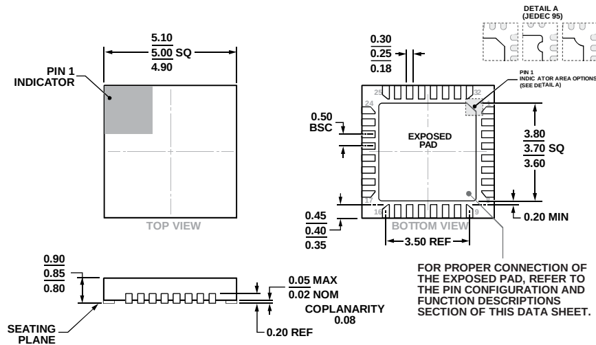
Figure 85. 32-Lead Lead Frame Chip Scale Package [LFCSP] 5 mm × 5 mm Body and 0.85mm Package Height (HCP-32-1)
