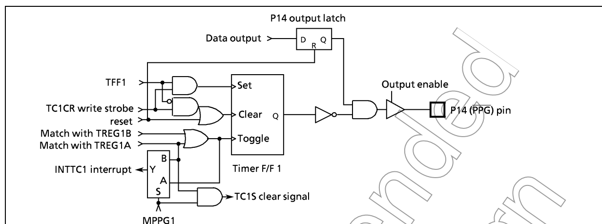
Figure 2-20. PPG Output
