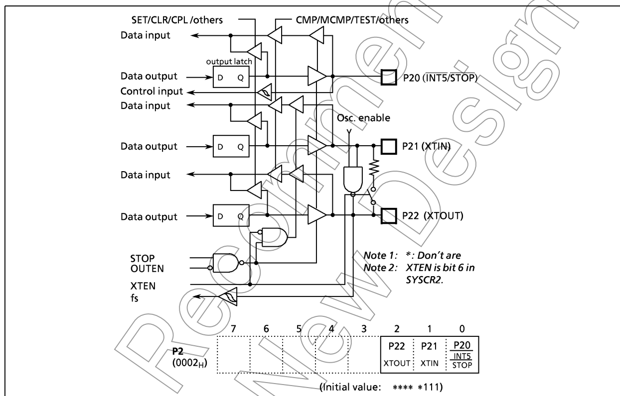
Figure 2-4. Port P2
