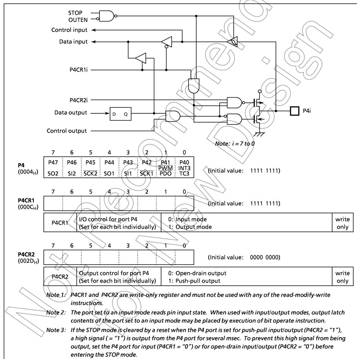
Figure 2-6. Port P4
