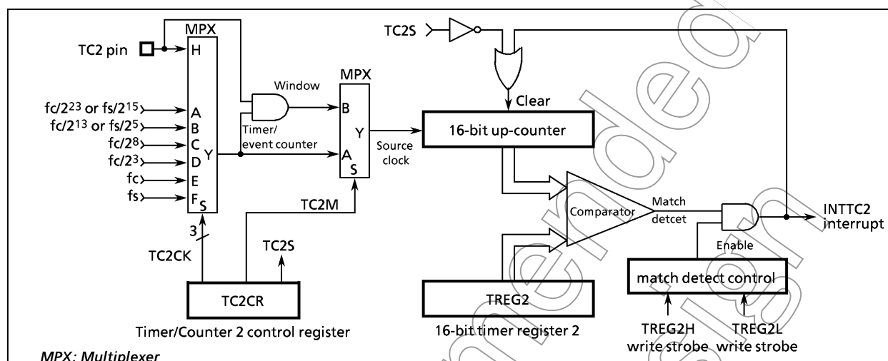
Figure 2-22. Timer/Counter 2 (TC2)
