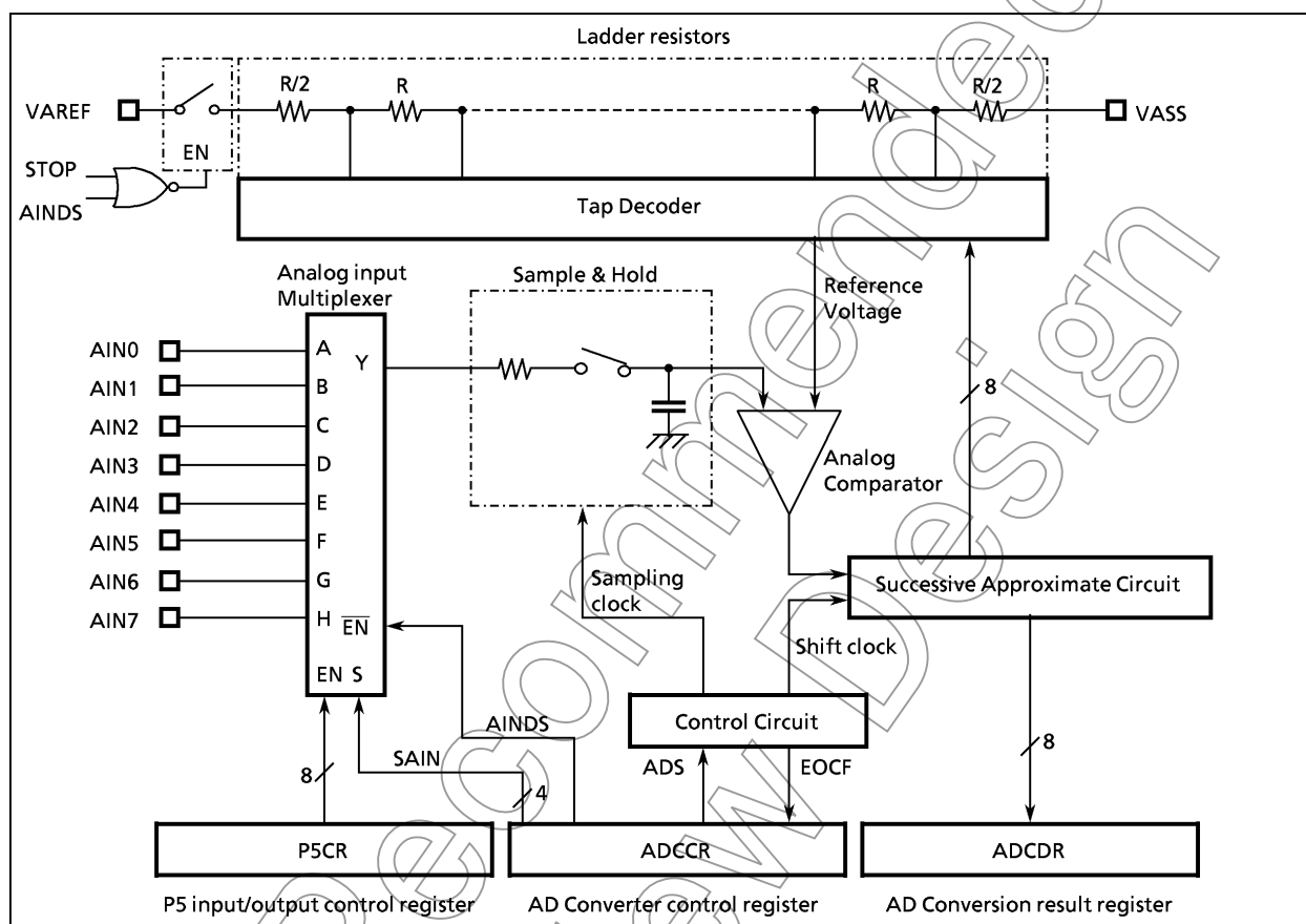
Figure 2-42. AD Converter
