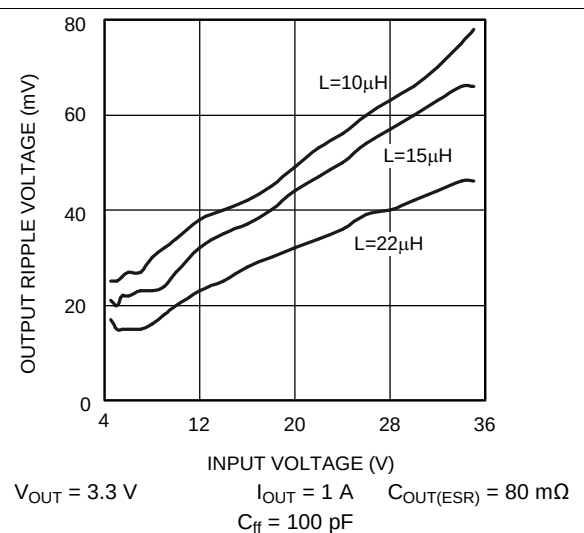
Figure 29. Output Ripple Voltage vs Input Voltage
