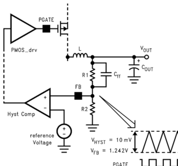
Figure 22. Hysteretic Window
