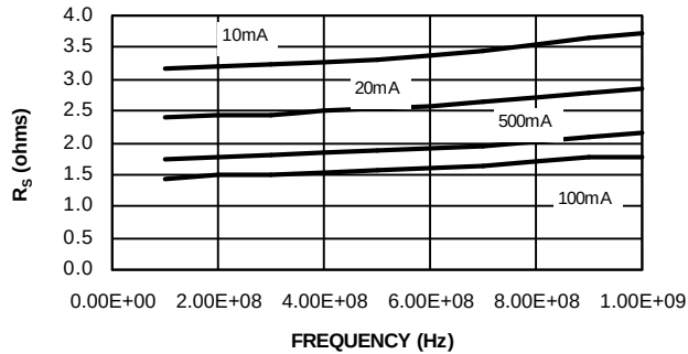
Typical Total Resistance R_S vs. Forward Current and Frequency
