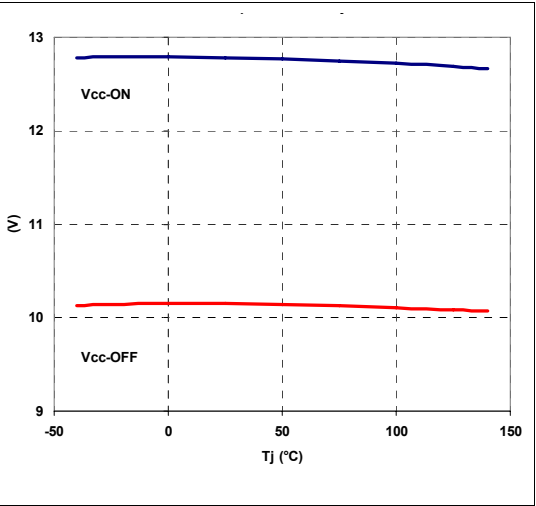
Figure 4. Start-up and UVLO vs T_j
