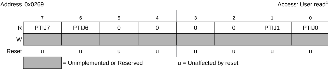
Figure 2-57. Port J Input Register (PTIJ)
