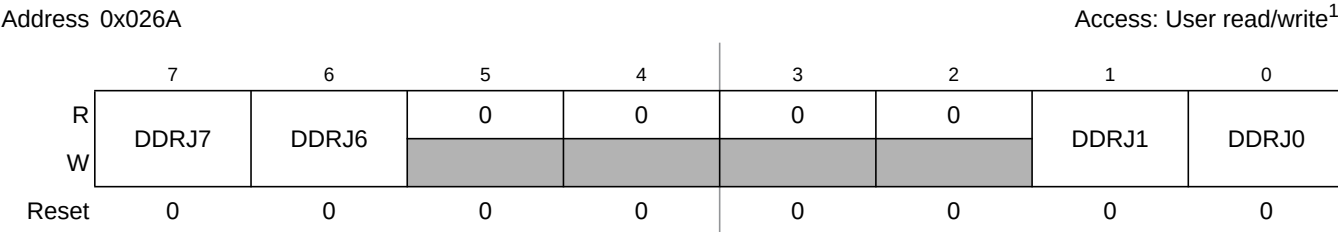
Figure 2-58. Port J Data Direction Register (DDRJ)
