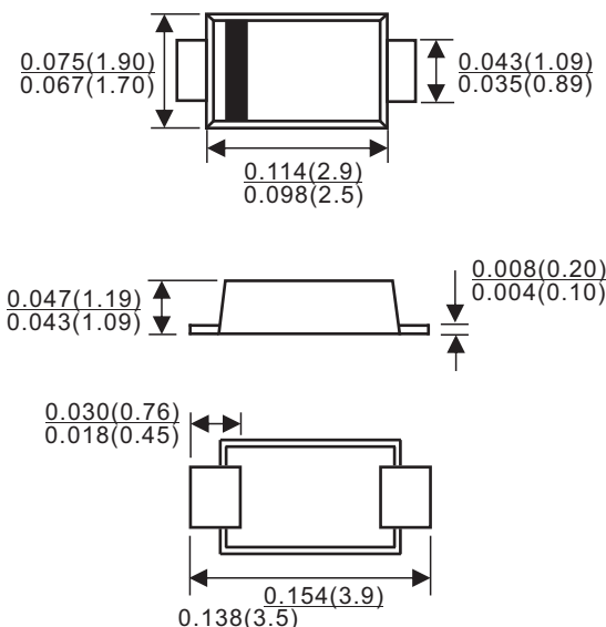
SOD-123FL
