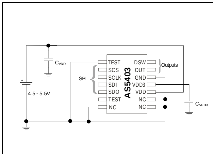
Figure 20: Connections for 5V Supply Voltages
