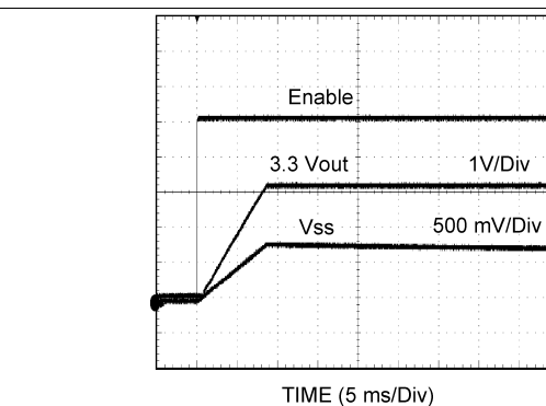
Figure 44. 3.3 V OUT Soft-Start
