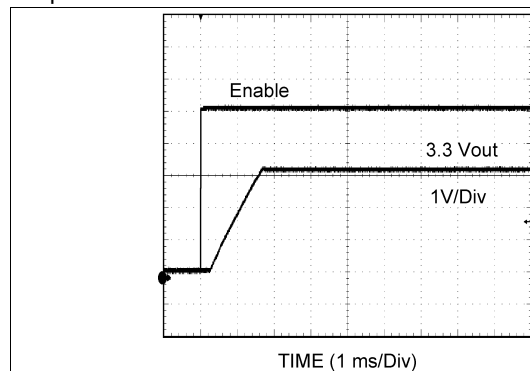
Figure 43. 3.3 V OUT Soft-Start
