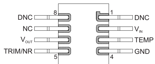
HKQ PACKAGE (TOP VIEW)
