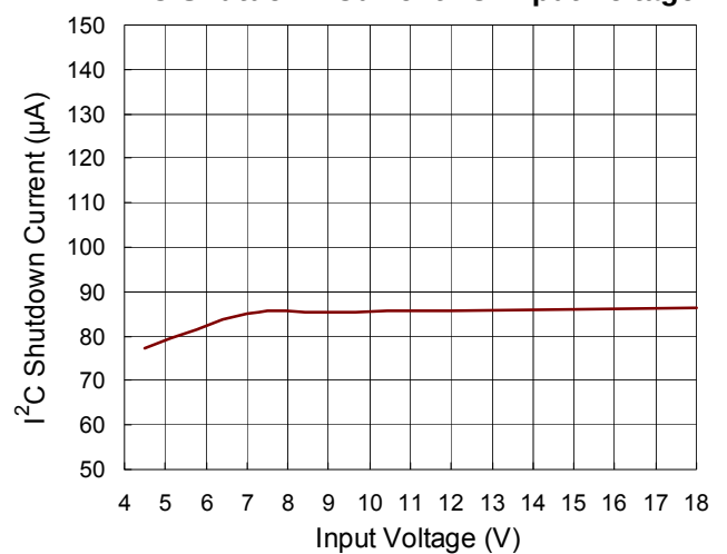
I^2C Shutdown Current vs. Input Voltage
