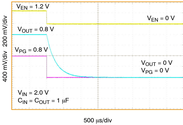
Figure 27. Turn-Off Response After De-asserting EN NCV8752A/B, V_{OUT} = 0.8\text{ V}
