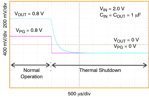
Figure 30. Turn-Off Response Due to Thermal Shutdown NCV8752A/B, V_{OUT} = 0.8\text{ V}
