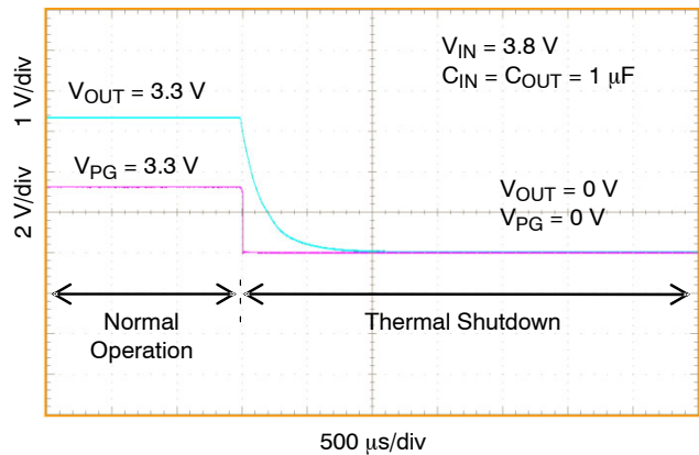
Figure 32. Turn-Off Response Due to Thermal Shutdown, V_{OUT} = 3.3\text{ V}
