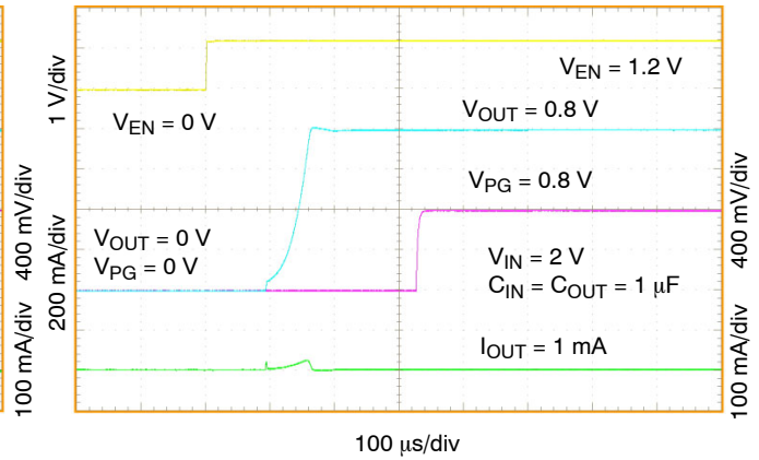
Figure 22. Turn-On Response After Asserting EN NCV8752B, V_{OUT} = 0.8 V
