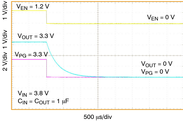
Figure 29. Turn-Off Response After De-asserting EN NCV8752A/B, V_{OUT} = 3.3\text{ V}
