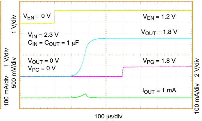
Figure 24. Turn-On Response After Asserting EN NCV8752B, V_{OUT} = 1.8 V
