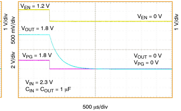
Figure 28. Turn-Off Response After De-asserting EN NCV8752A/B, V_{OUT} = 1.8\text{ V}
