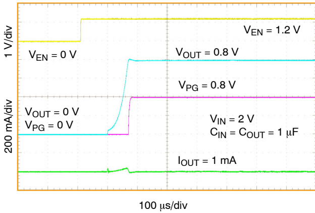
Figure 21. Turn-On Response After Asserting EN NCV8752A, V_{OUT} = 0.8 V
