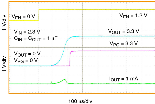
Figure 25. Turn-On Response After Asserting EN NCV8752A, V_{OUT} = 3.3 V
