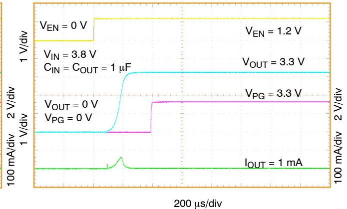
Figure 26. Turn-On Response After Asserting EN NCV8752B, V_{OUT} = 3.3 V
