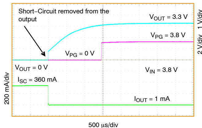
Figure 50. Recovery from Short-Circuit NCV8752B, V_{OUT} = 3.3 \text{ V}
