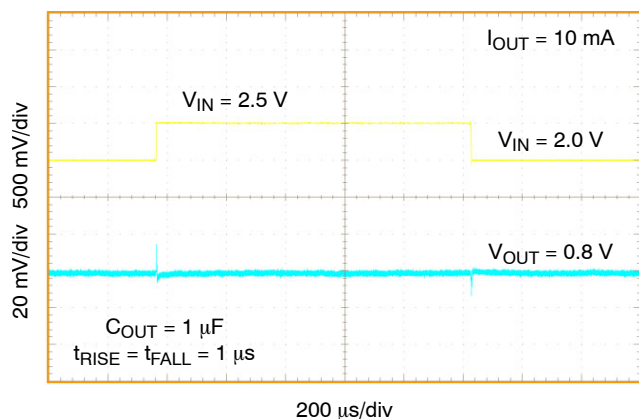
Figure 51. Line Transient 2 V – 2.5 V NCV8752A/B, V_{OUT} = 0.8 V
