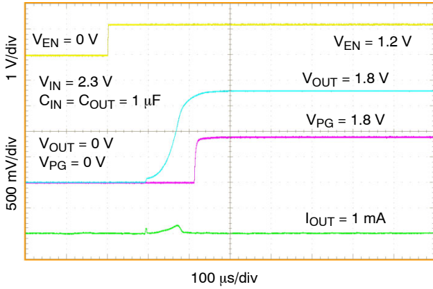
Figure 23. Turn-On Response After Asserting EN NCV8752A, V_{OUT} = 1.8 V
