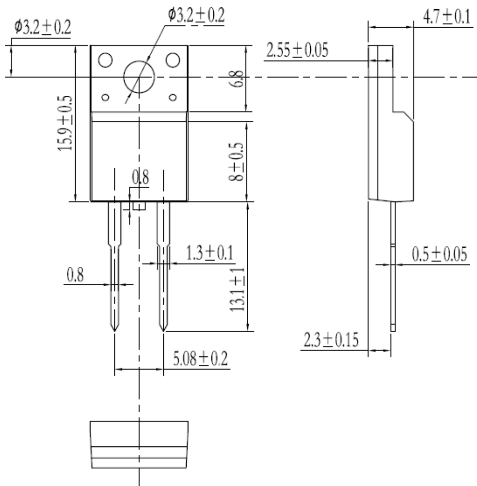
Dimensions in (mm) Figure 8. Package Outline
