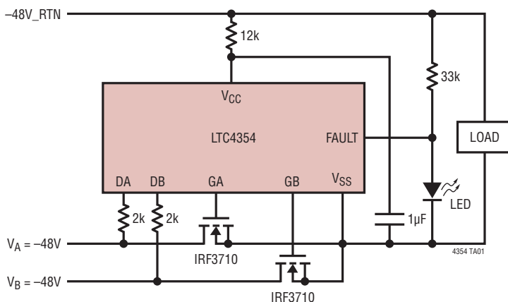
-48V Diode-OR
