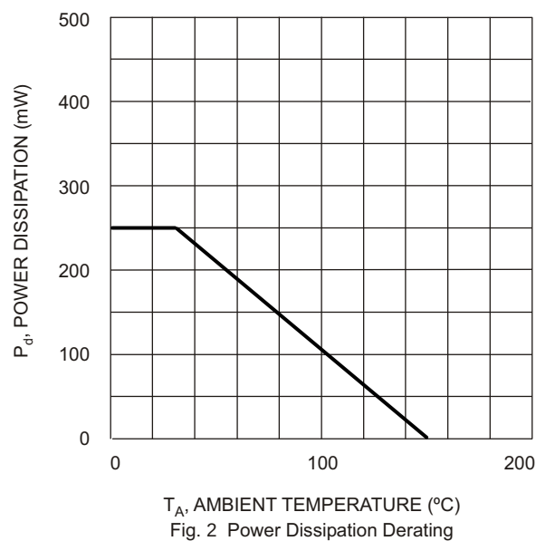
Fig. 2 Power Dissipation Derating
