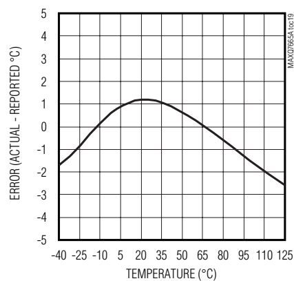
EXTERNAL DIODE TEMPERATURE-SENSOR ERROR vs. TEMPERATURE
