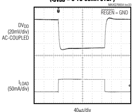
DV_{DD} LINEAR REGULATOR OUTPUT VOLTAGE LOAD TRANSIENT ( I_{DDDD} = 0 TO 50mA STEP)
