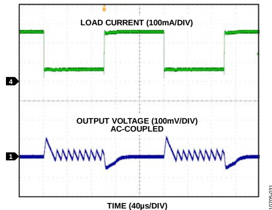
Figure 18. Load Transient Response, V_{OUT} = 1.8 V, Auto Mode, 50 mA to 250 mA
