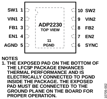
Figure 2. Pin Configuration
