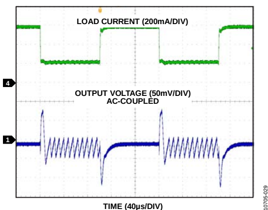
Figure 16. Load Transient Response, V_{OUT} = 1.2 V, Auto Mode, 200 mA to 600 mA
