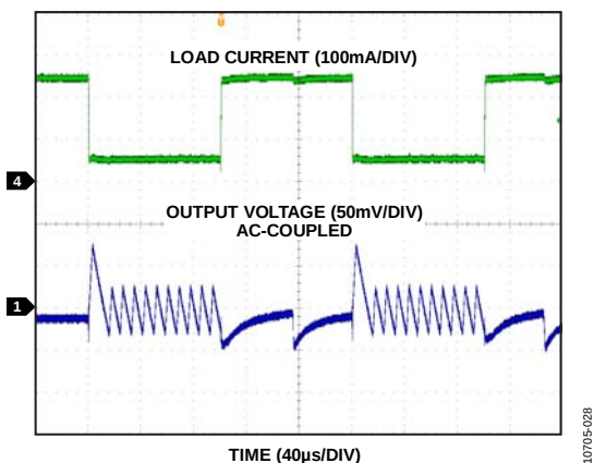
Figure 15. Load Transient Response, V_{OUT} = 1.2 V, Auto Mode, 50 mA to 250 mA
