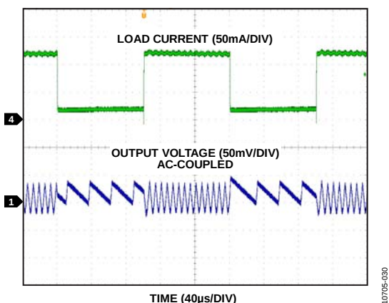
Figure 17. Load Transient Response, V_{OUT} = 1.8 V, Auto Mode, 10 mA to 110 mA
