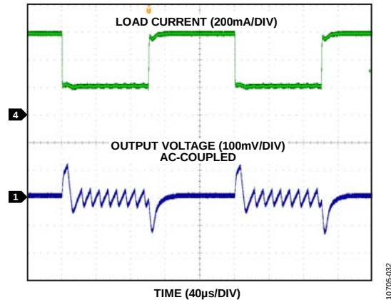
Figure 19. Load Transient Response, V_{OUT} = 1.8 V, Auto Mode, 200 mA to 600 mA
