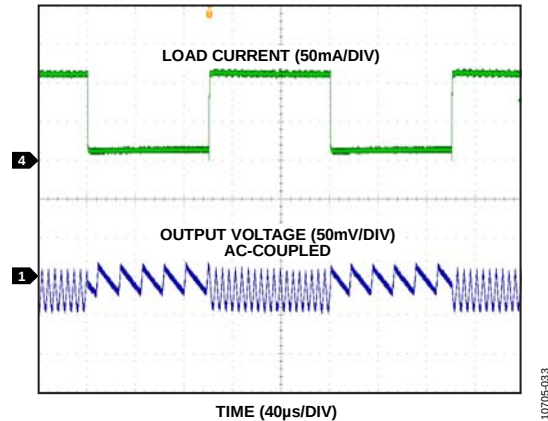
Figure 20. Load Transient Response, V_{OUT} = 3.3 V, Auto Mode, 10 mA to 110 mA
