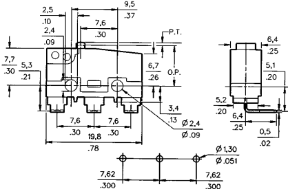
PC Right Angle In-line – Type 50
