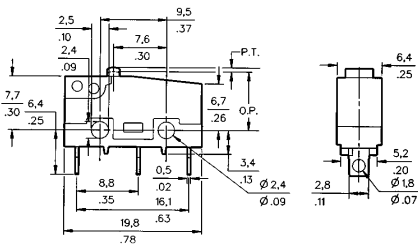
PC Right Angle In-line – Type 50
