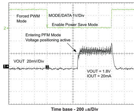
Figure 33. Forced PWM/PFM Mode Transition
