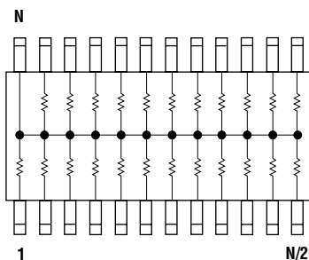
NQS16B, NQS20B, NQS24B Bussed Resistors
