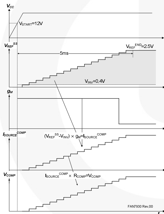
Figure 34. Soft-Start Sequence
