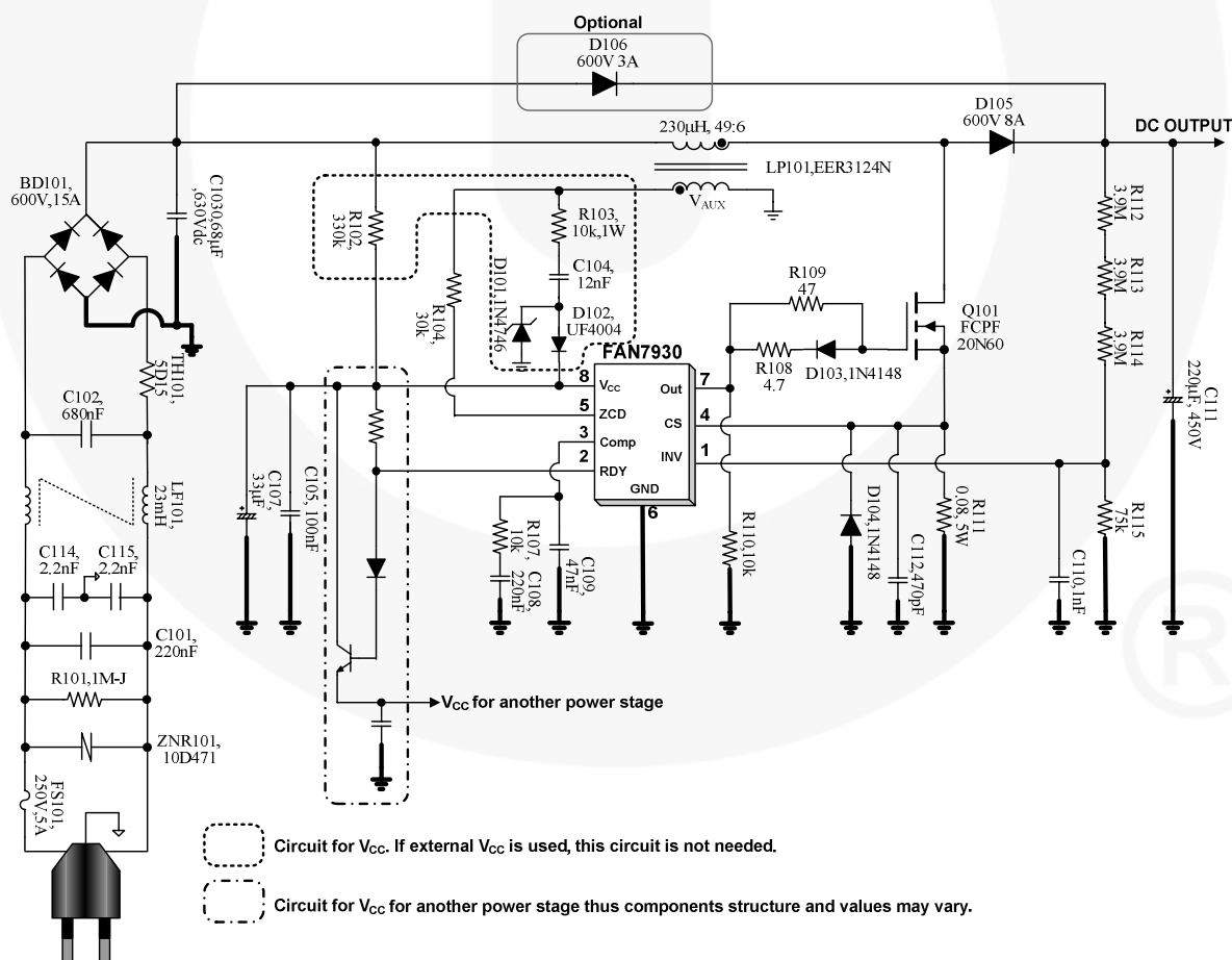
Figure 43. Demonstration Circuit
