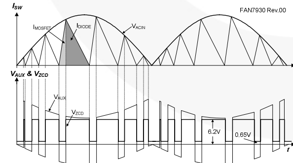
Figure 26. Auxiliary Voltage Depends on MOSFET Switching
