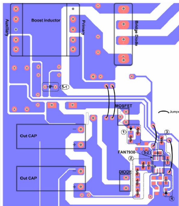
Figure 42. Recommended PCB Layout
