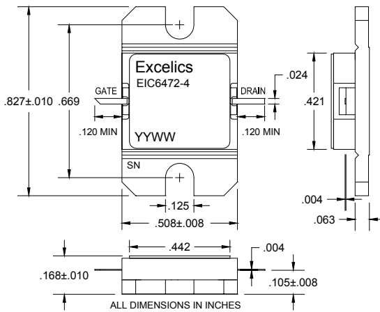
EIC6472-4 (Hermetic)
