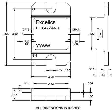
EIC6472-4NH (Non-Hermetic)
