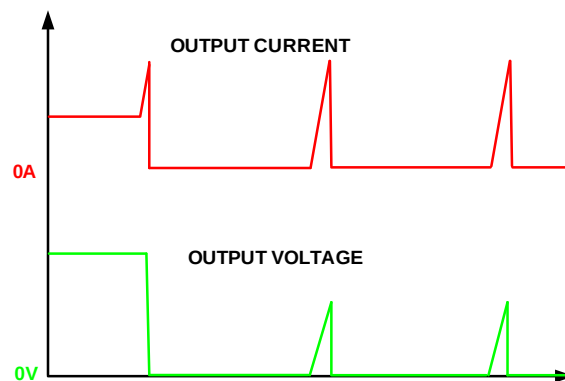
Figure 9—Over-current Behavior in HICCUP Mode. F_{\text{sw}} = 600\text{kHz}
