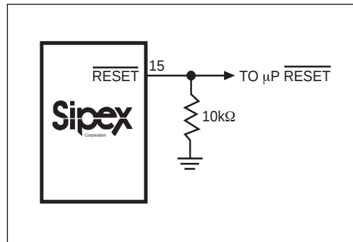
Figure 18. External Pull-down Resistor Ensures \overline{RESET} is Valid with V_{CC} Down to Ground.
