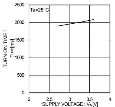
Fig.20 Output turn on time
