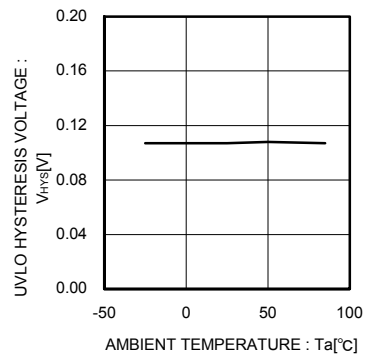
Fig.27 UVLO hysteresis voltage
