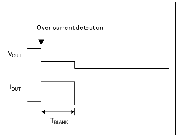
Fig.3 Over current limits characteristics
