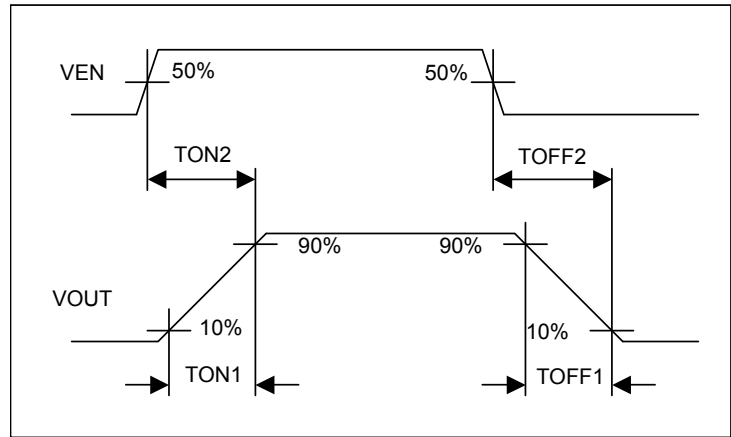
Fig.2 Switch Turn on / off time
