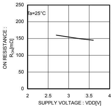
Fig.10 ON resistance
