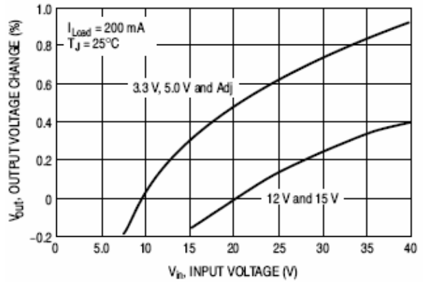
Figure 3. Line Regulation
