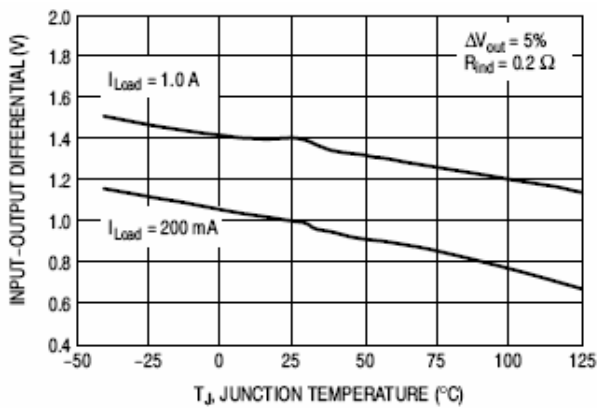
Figure 6. Dropout Voltage
