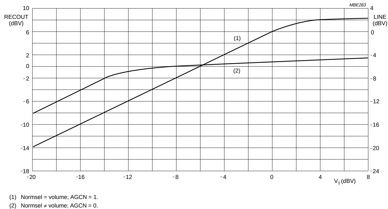
Fig.11 RECOUT/LINE output as a function of audio signal level (hi-fi inputs).
