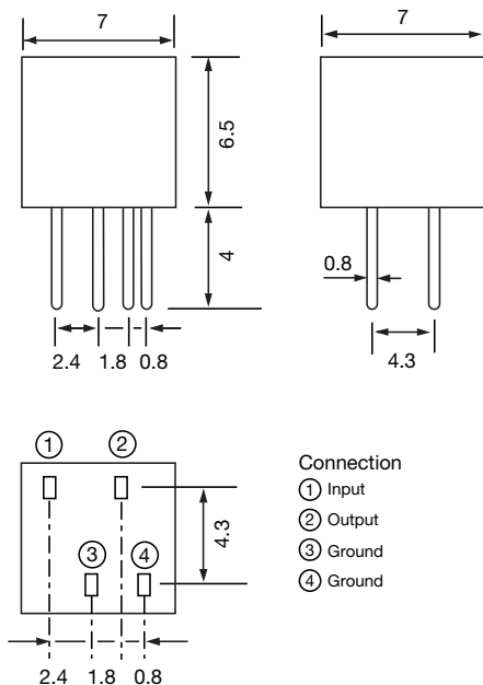
Figure 1) LTM450U – Front, Side and Bottom views
