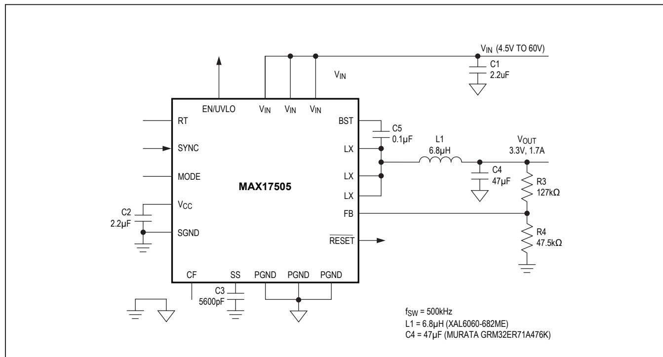
Figure 4. MAX17505 Typical Application Circuit (3.3V, 500kHz Switching Frequency)
