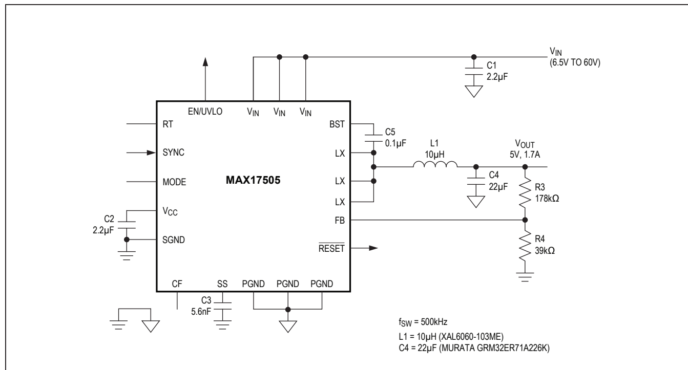
Figure 3. MAX17505 Typical Application Circuit (5V, 500kHz Switching Frequency)
