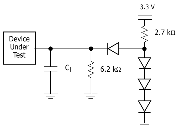
Figure 9. Test Setup
